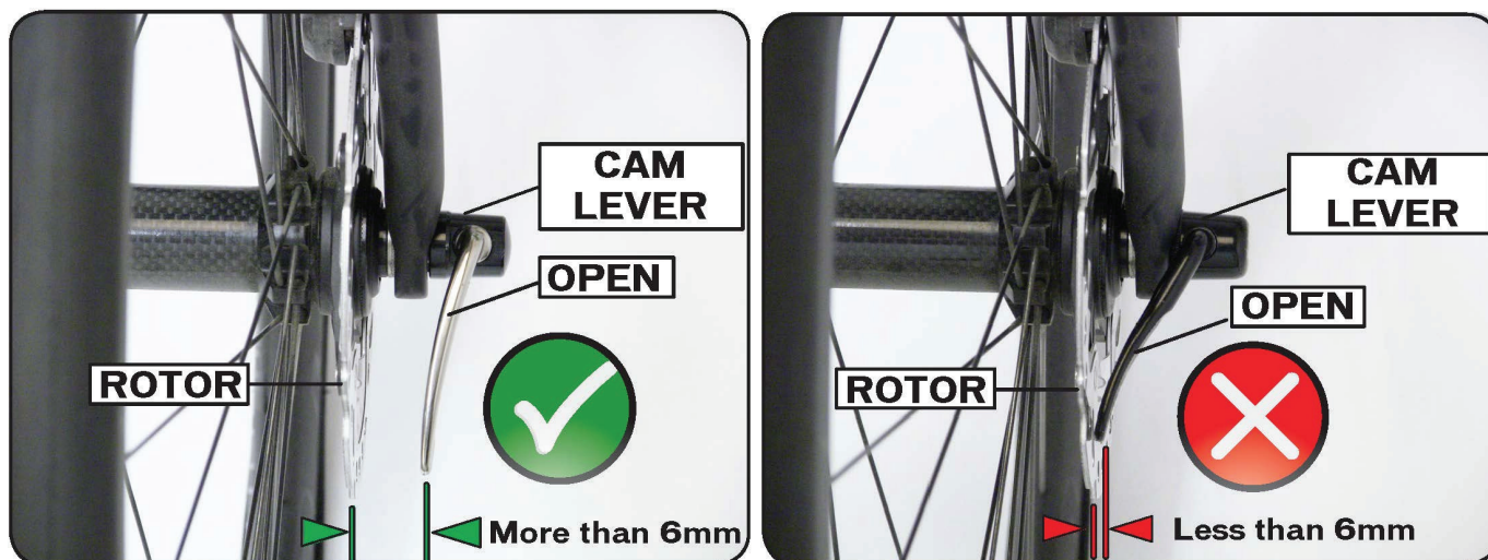
Fig1: Quick Release not affected by this recall
